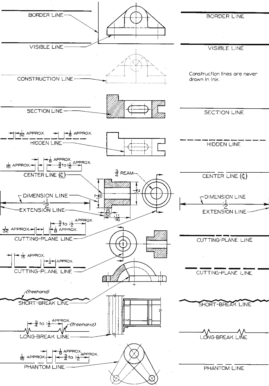
Fig. 3-11. Alphabet of Lines.
