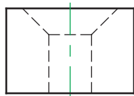
Countersink
