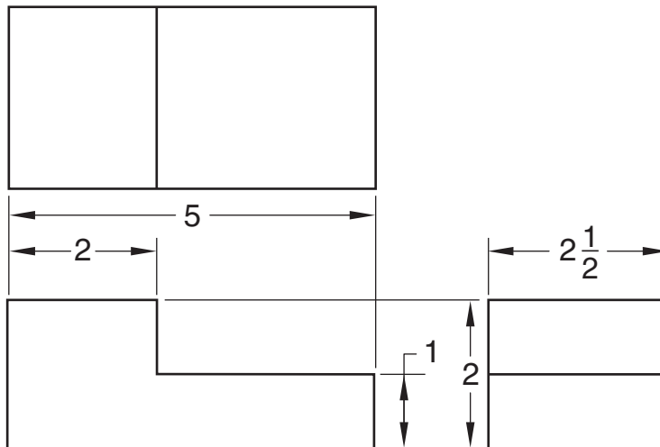
Unidirectional Dimensioning (Preferred)
