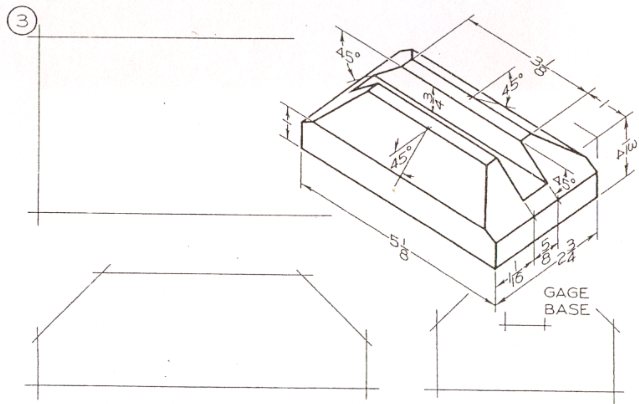
Fig. 7-31. Working Drawing Problems. Using Layout C (Appendix, page 474), make mechanical drawings. Omit dimensions unless assigned. Omit pictorial drawings. Move titles to title strip.
